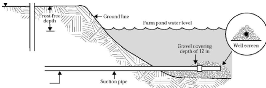
Figure 6 Details of a dry hydrant installation
